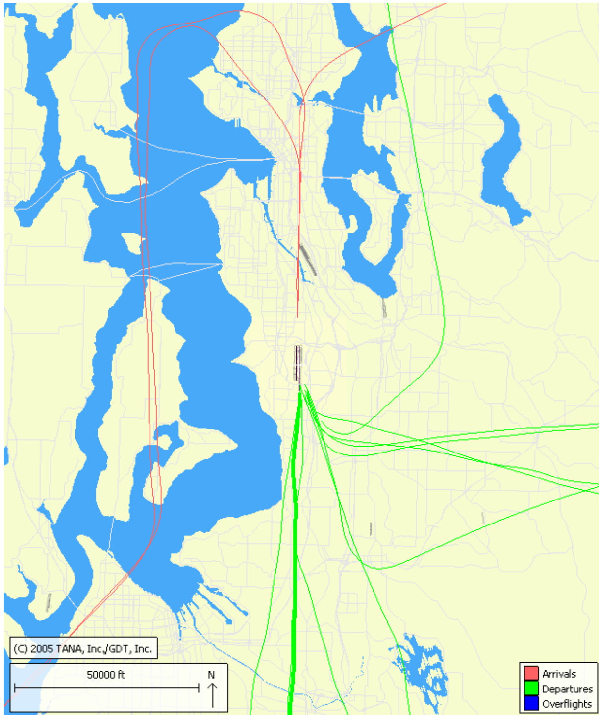
Sea-Tac Aircraft Sample Flight Track Pattern South Flow Props 10:00 p.m. to 6:00 a.m.
